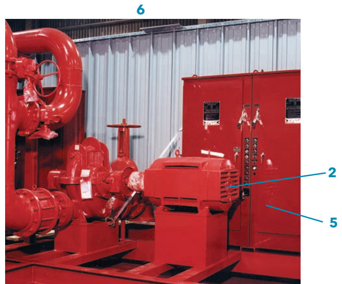
This system includes three electric motor driven fire pumps, 16' x 53' and weighs 57,000 lbs.
